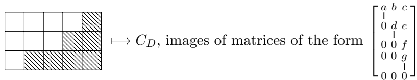
FIGURE 1. A Young diagram d \subset [0, n - k] \times [0, k] determines a Schubert cycle C_D \subset \text{Gr}(k, n) . The diagram consists of the unshaded squares. Each vertical edge corresponds to a special pivot row of the matrix; other rows have a certain number of free variables. The class \sigma_D is represented by C_D .
